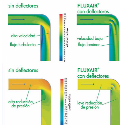
CODO VERTICAL
